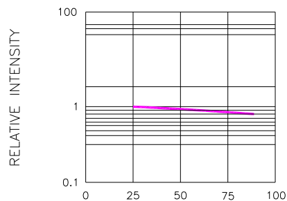
Fig.3 RELATIVE INTENSITY VS. LEAD TEMPERATURE (PULSED 20 mA; 300 \mu s PULSE, 10ms PERIOD)
