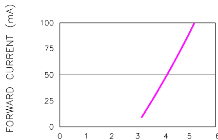
Fig.4 PEAK FORWARD VOLTAGE VS. FORWARD (100 \mu s TEST PULSE, 1% DUTY CYCLE)
