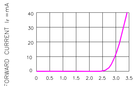
Fig.2 FORWARD CURRENT VS. FORWARD VOLTAGE
