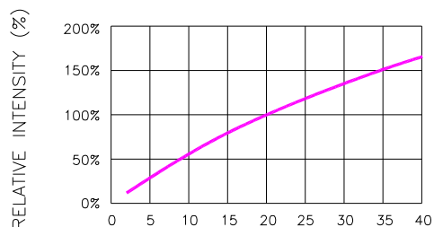
Fig.1 RELATIVE INTENSITY VS. FORWARD CURRENT
