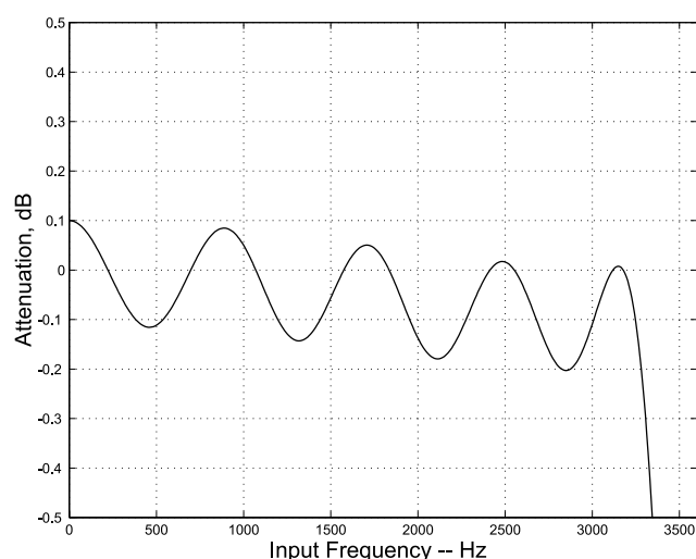
Figure 10. FIR Transmit Filter Passband Ripple
