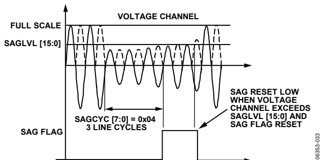
Figure 57. SAG Detection
