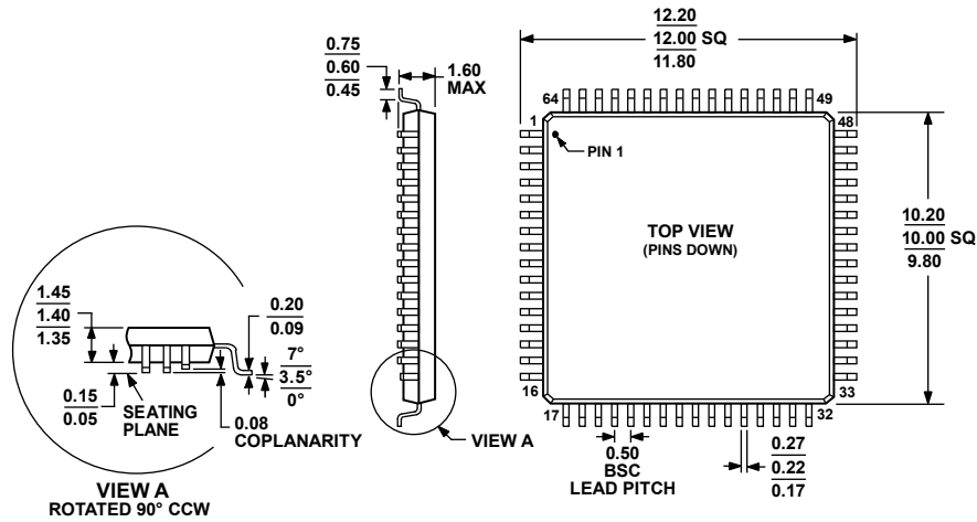
Figure 118. 64-Lead Low Profile Quad Flat Package [LQFP] (ST-64-2)
