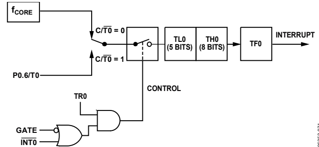
Figure 97. Timer/Counter 0, Mode 0
