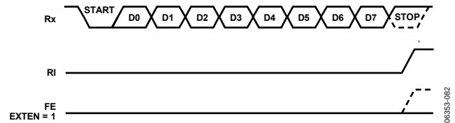
Figure 108. UART Timing in Mode 1
