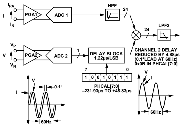
Figure 59. Phase Calibration
