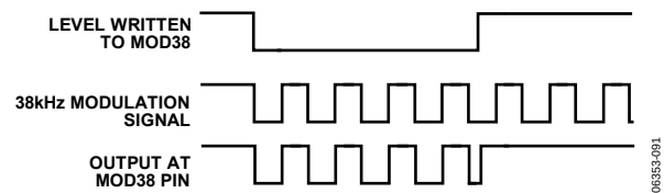
Figure 117. 38 kHz Modulation
