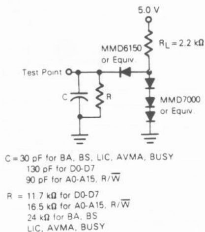
FIGURE 4 — BUS TIMING TEST LOAD
