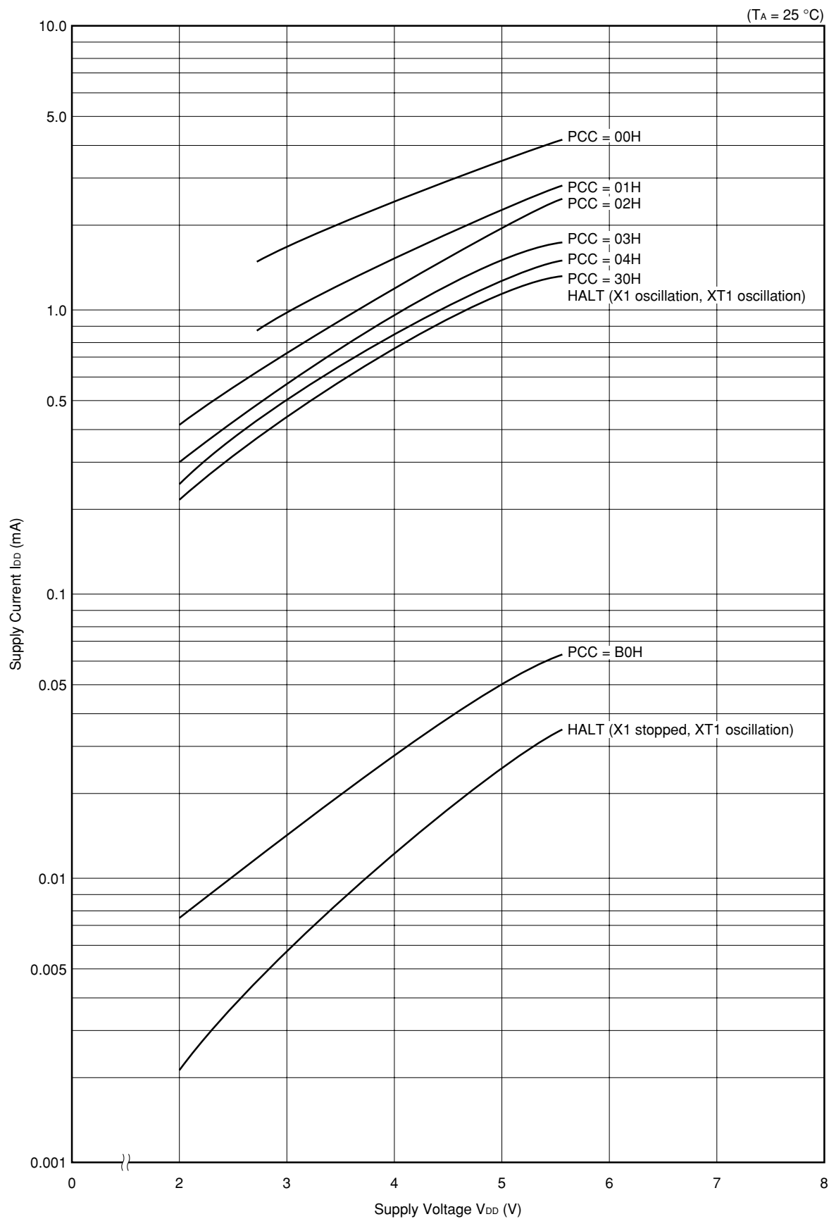
I_{DD} vs V_{DD} ( f_x = 5.0 MHz, f_{xx} = 2.5 MHz)
