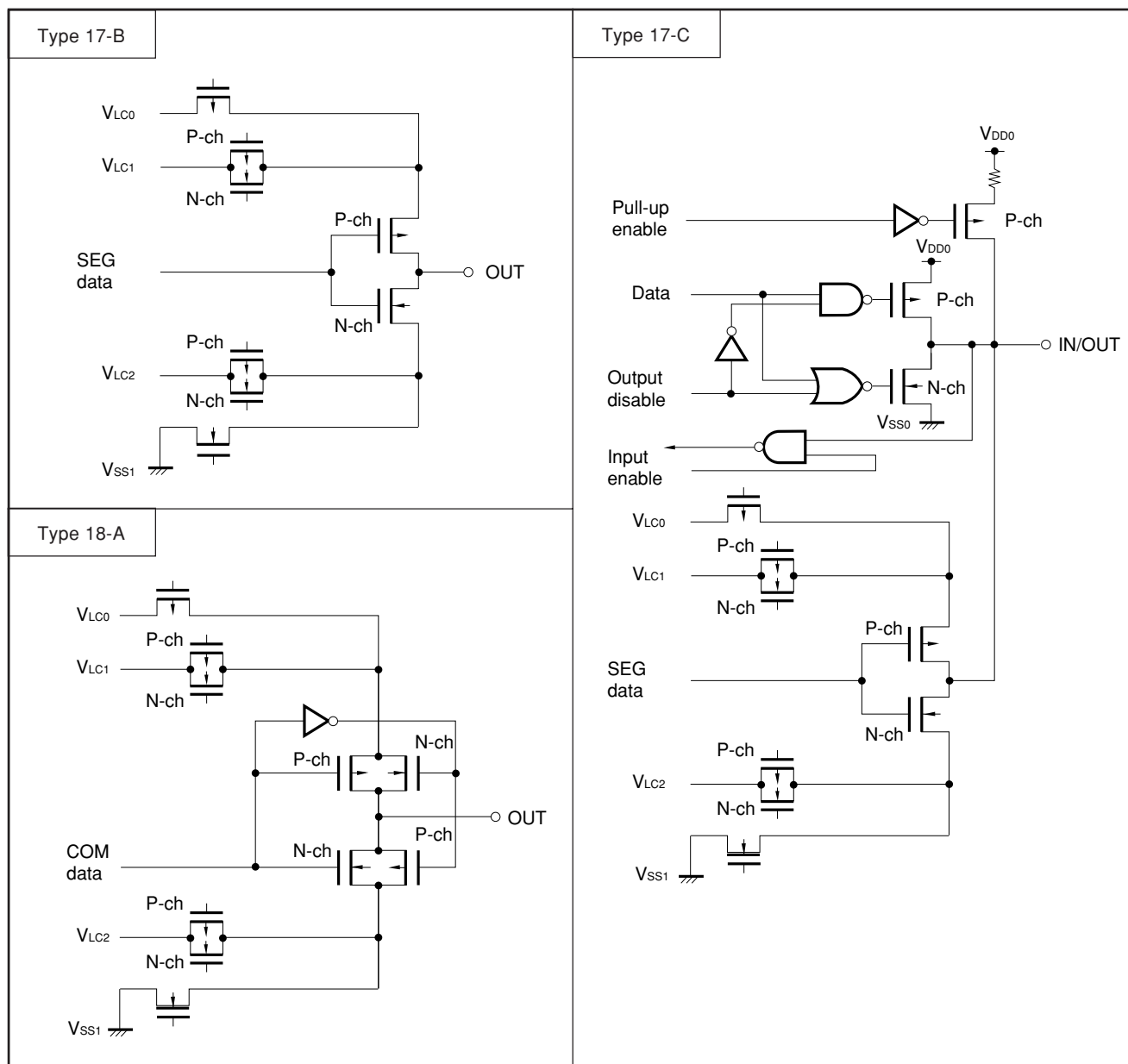
Figure 3-1. Pin Input/Output Circuits (2/2)
