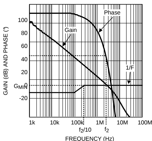
Figure 59. LMP7707 Open Loop Gain and 1/F Lead-Lag Feedback Network.
