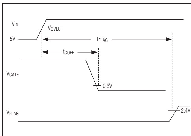
Figure 2. Shutdown Timing Diagram
