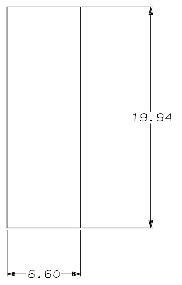
RECOMMENDED CUT OUT FOR 1.52 MAX THICK PANEL
