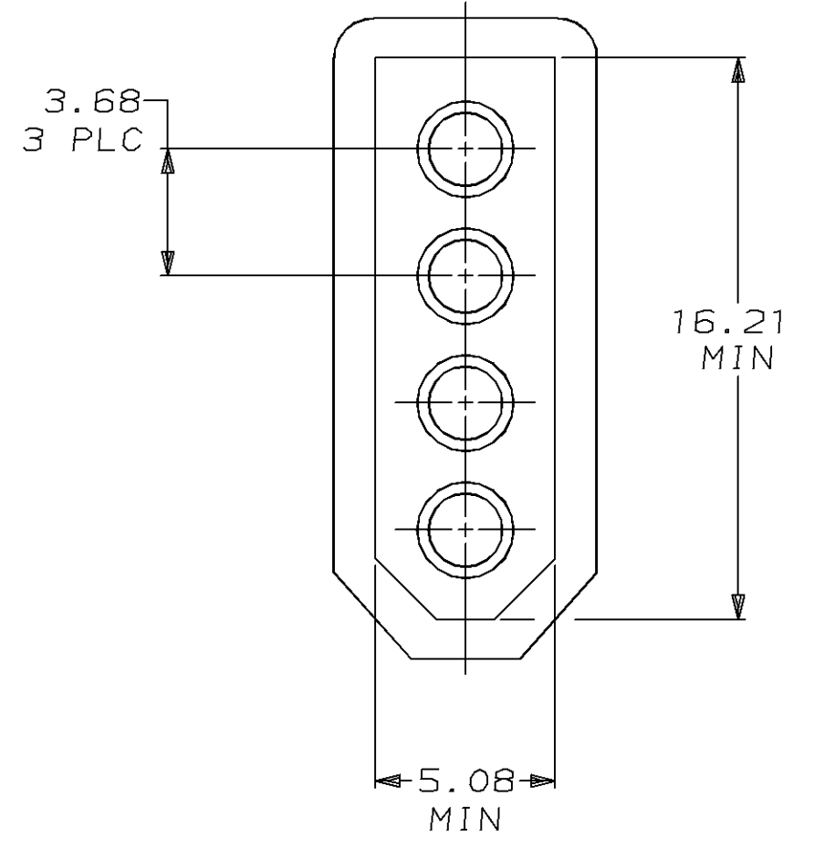
MATING CONNECTOR INTERFACE
