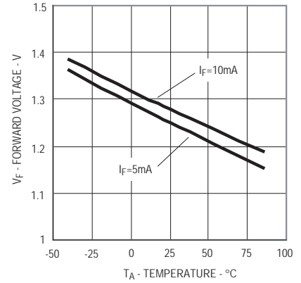
Figure 6. Typical Forward Voltage vs. Temperature
