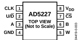
Figure 5. SOT-23-8 Pin Configuration
