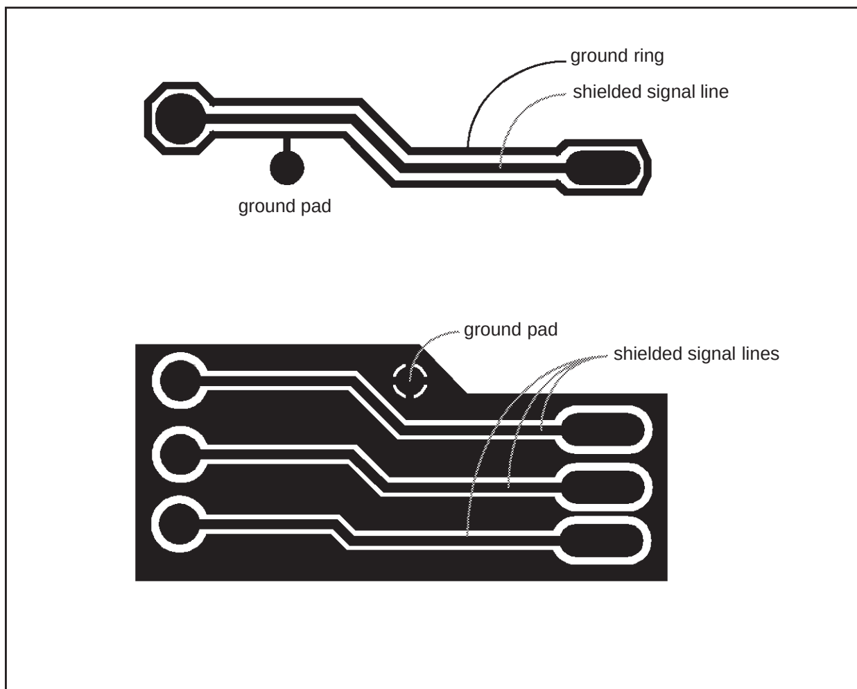
Figure 6-8. Shielding signals
