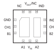
4x4mm 12-Lead MLP(QUAD) (Internal Schottky Diode)
