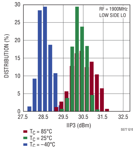
1900MHz IIP3 Distribution
