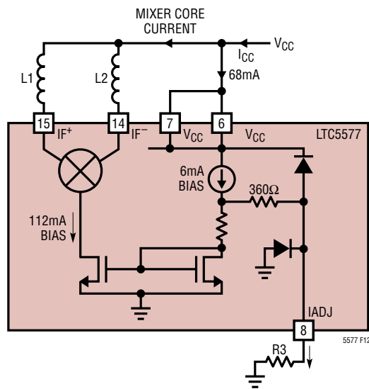
Figure 12. IADJ Interface
