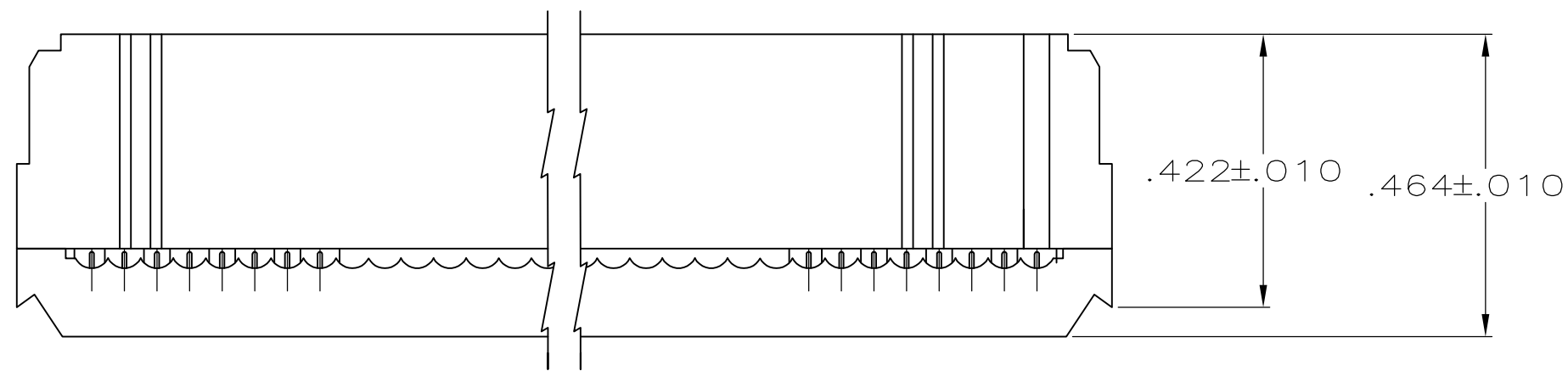
TERMINATED VIEW
