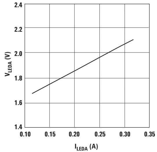
Figure 10. V_{LED} vs I_{LED} .
