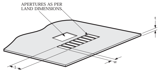
Figure 14. Solder stencil aperture.
