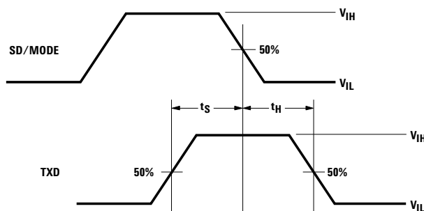
Figure 4. Bandwidth selection timing at FIR mode.
