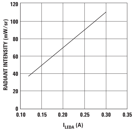
Figure 9. Radiant Intensity vs I_{LED} .
