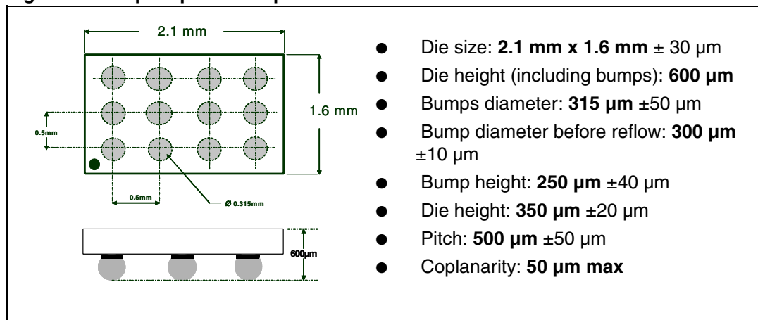
Figure 46. Flip-chip - 12 bumps
