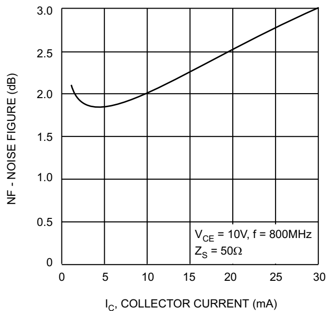
Fig 4. Noise Figure vs. Collector Current
