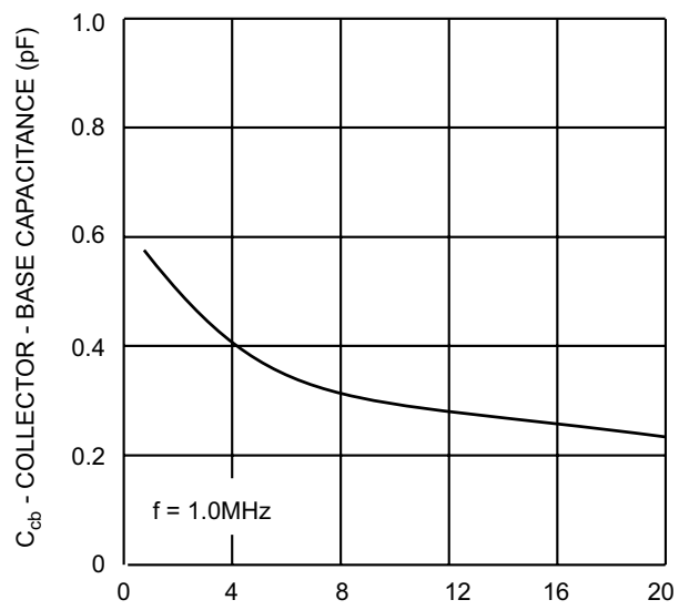
Fig. 2 Collector - Base Capacitance vs. Collector - Base Voltage
