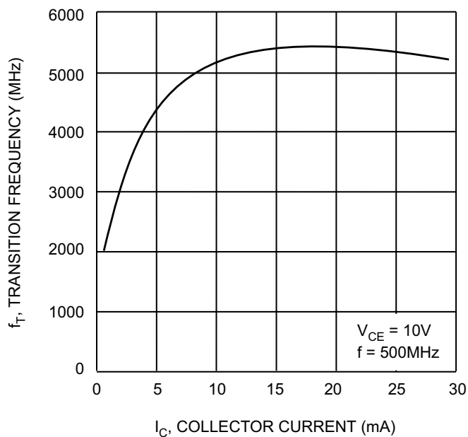
Fig 3. Transition Frequency vs. Collector Current
