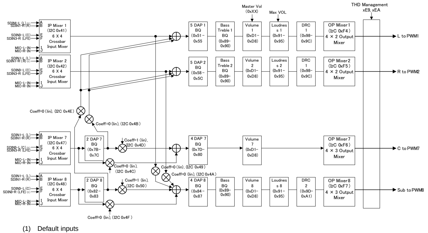
Figure 24. TAS5548 Architecture With I²C Registers in 192kHz Native Mode ( f_s = 176.4 \text{ kHz} or f_s = 192 \text{ kHz} )
