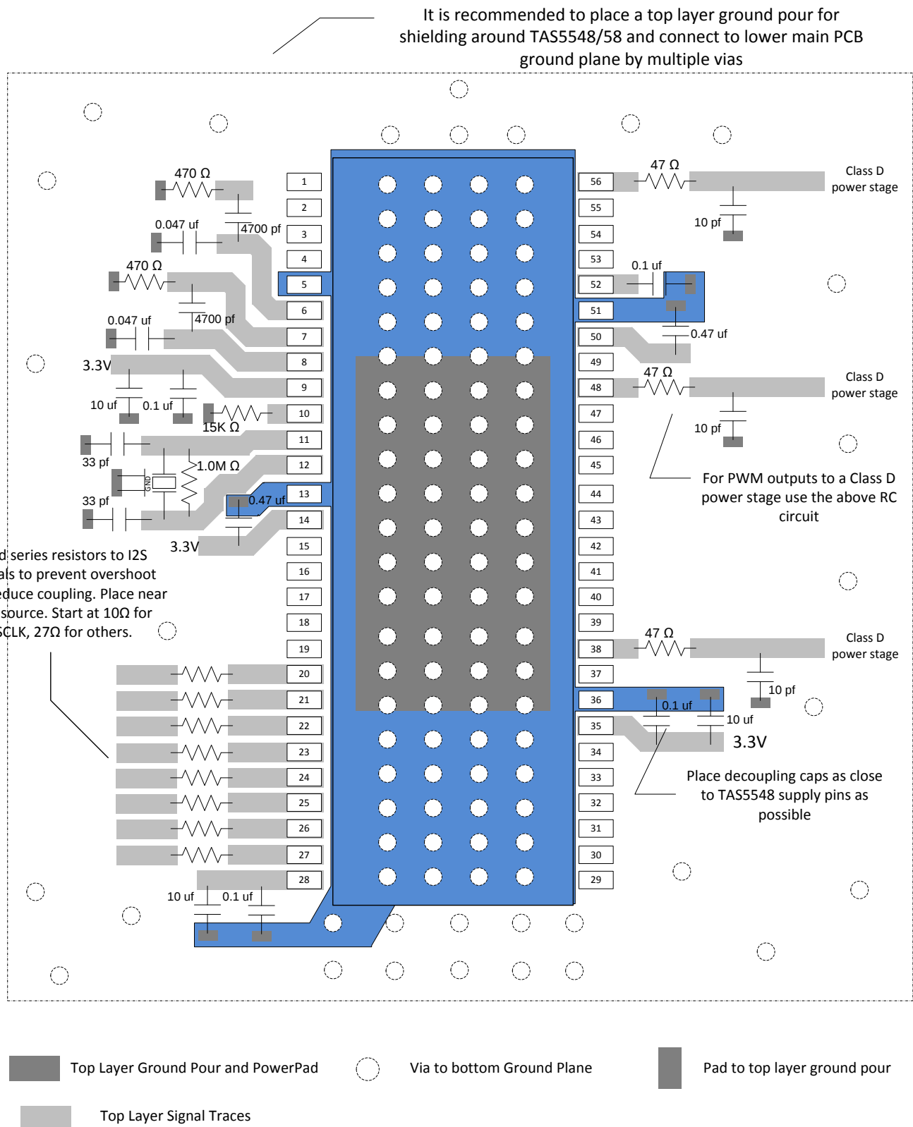
Figure 53. TAS5548 Layout Example
