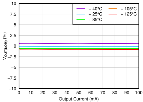
Figure 6-7. Load Regulation
