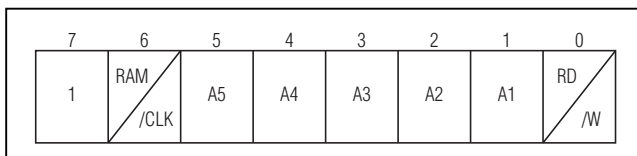
Figure 24. Address/Command Byte
