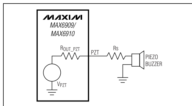
Figure 16. Piezo Transducer Functional Diagram
