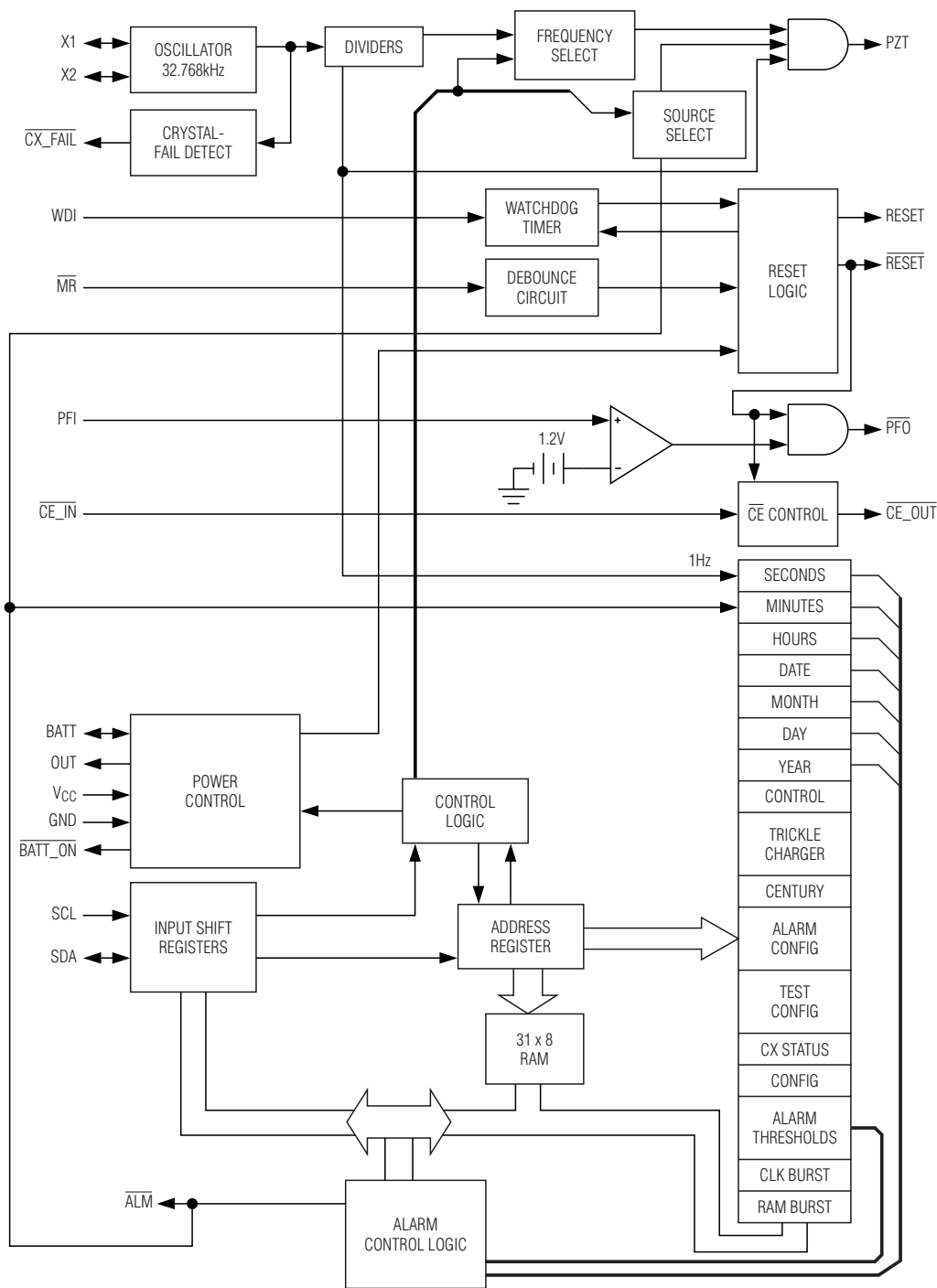
Figure 1. MAX6909/MAX6910 Block Diagram
