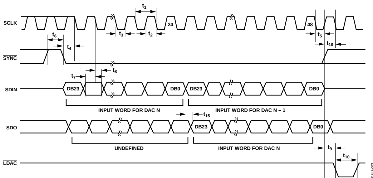
Figure 4. Daisy-Chain Timing Diagram
