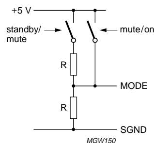
Fig.3 Mode select switch circuitry.
