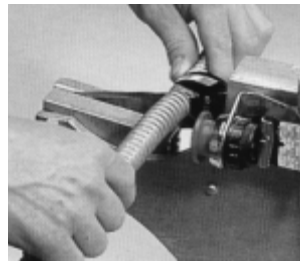
Cut through the helix with pliers
