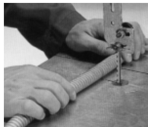
Position conduit at right-angle to band saw
