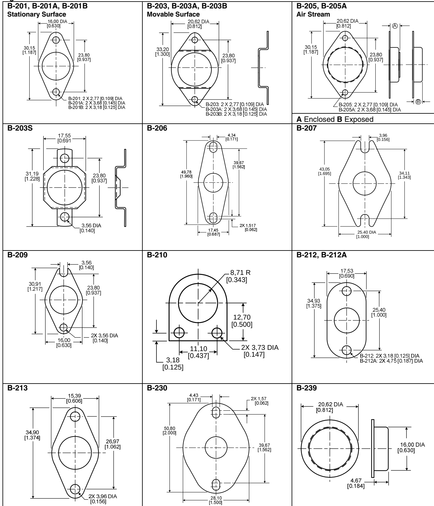
Figure 19. Brackets
