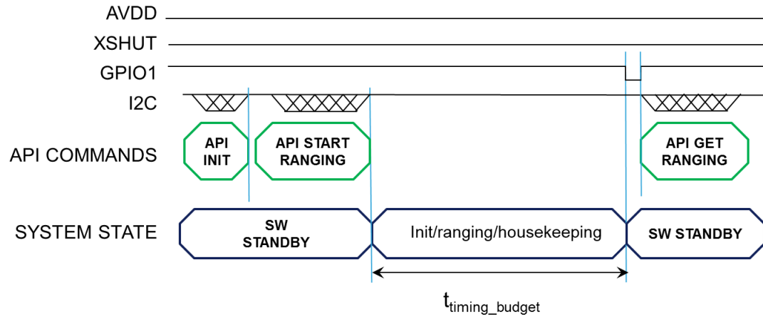
Figure 8. Ranging sequence
