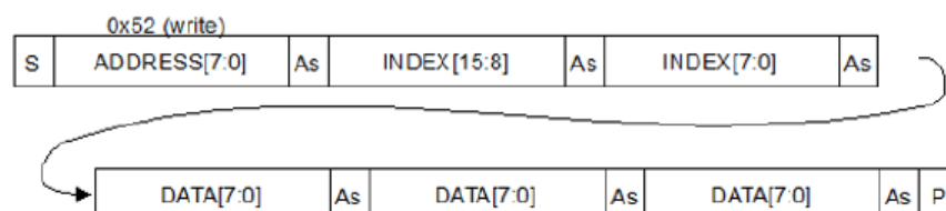
Figure 13. Data format (sequential write)
