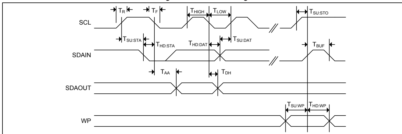
Figure 5-11. Bus Timing
