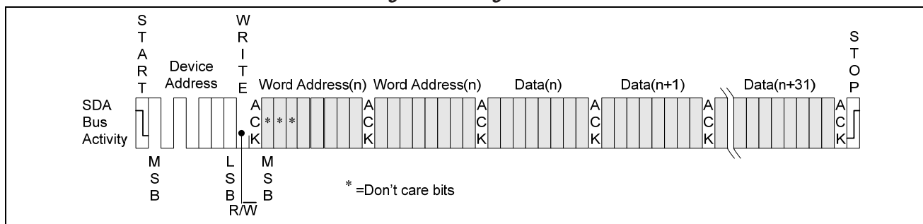
Figure 5-7. Page Write
