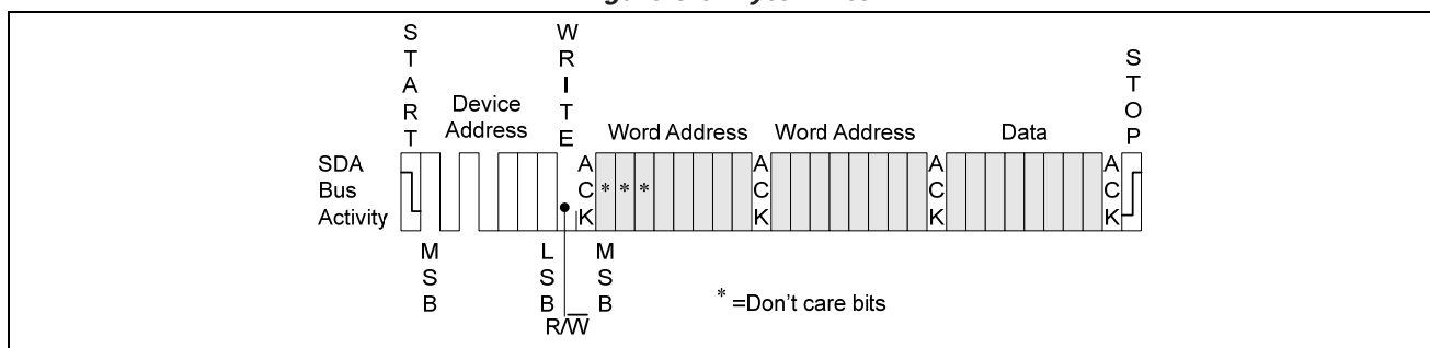
Figure 5-6. Byte Write
