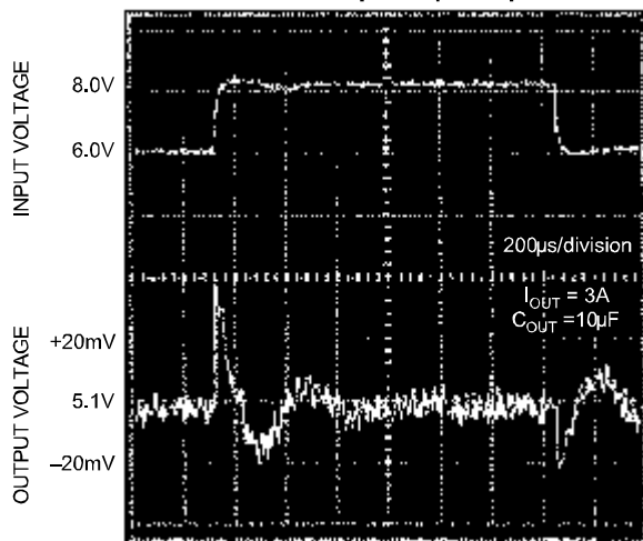
Line Transient Response with 3A Load, 10\mu F Output Capacitance
