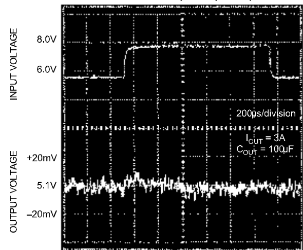
Line Transient Response with 3A Load, 100\mu F Output Capacitance
