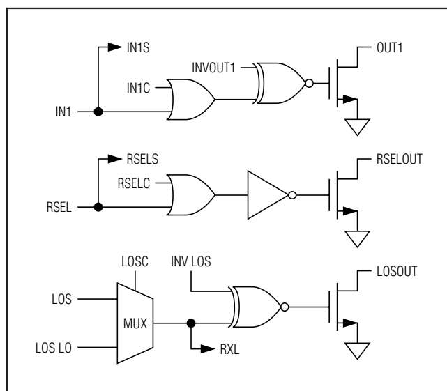
Figure 13. Logic Diagram 2
