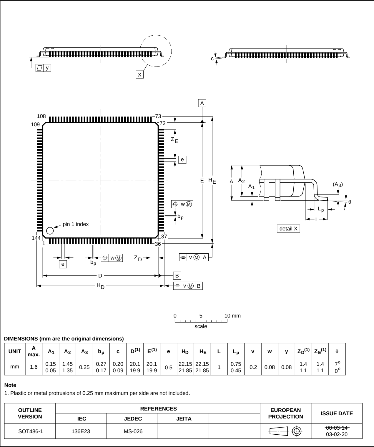
Fig 44. LQFP144 package
