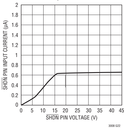
\overline{\text{SHDN}} Pin Input Current
