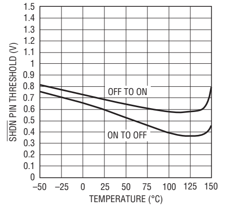
\overline{\text{SHDN}} Pin Thresholds
