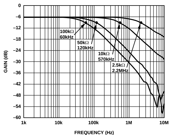
Figure 20. -3 dB Bandwidth @ Code = 0x80
