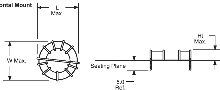
Figure 2 Horizontal Mount
