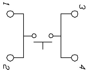
CONTACT CONFIGURATION
