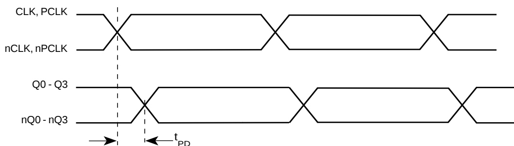
FIGURE 6 - PROPAGATION DELAY
