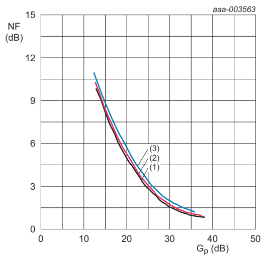
GS1 = LOW; GS2 = HIGH; V_{CC1} = 5\text{ V} ; V_{CC2} = 5\text{ V} ; f = 1950\text{ MHz} . (1) T_{amb} = -10\text{ }^{\circ}\text{C} (2) T_{amb} = +25\text{ }^{\circ}\text{C} (3) T_{amb} = +85\text{ }^{\circ}\text{C}
