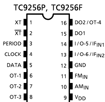
Top View DIP-16PIN / SOP-16PIN
