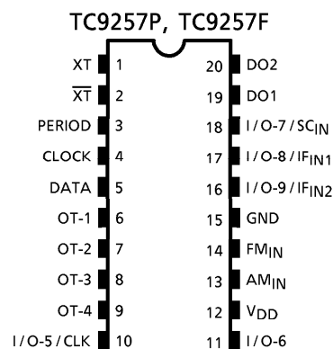
Top View DIP-20PIN / SOP-20PIN
