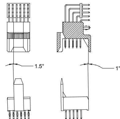
INCLINATION TOLERANCES
