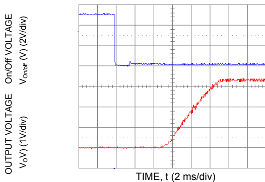
Figure 15. Typical Start-Up Using Remote On/Off with Low-ESR external capacitors (7x150µF Polymer) ( V_{in} = 5.0\text{Vdc} , V_o = 3.3\text{Vdc} , I_o = 6\text{A} , C_o = 1050\text{ }\mu\text{F} ).
