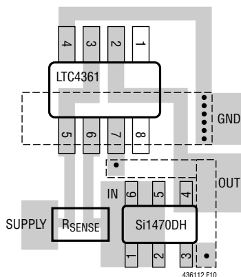
Figure 10. Layout for N-Channel MOSFET Configuration
