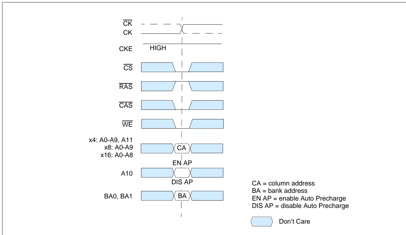
Figure 16 Write Command
