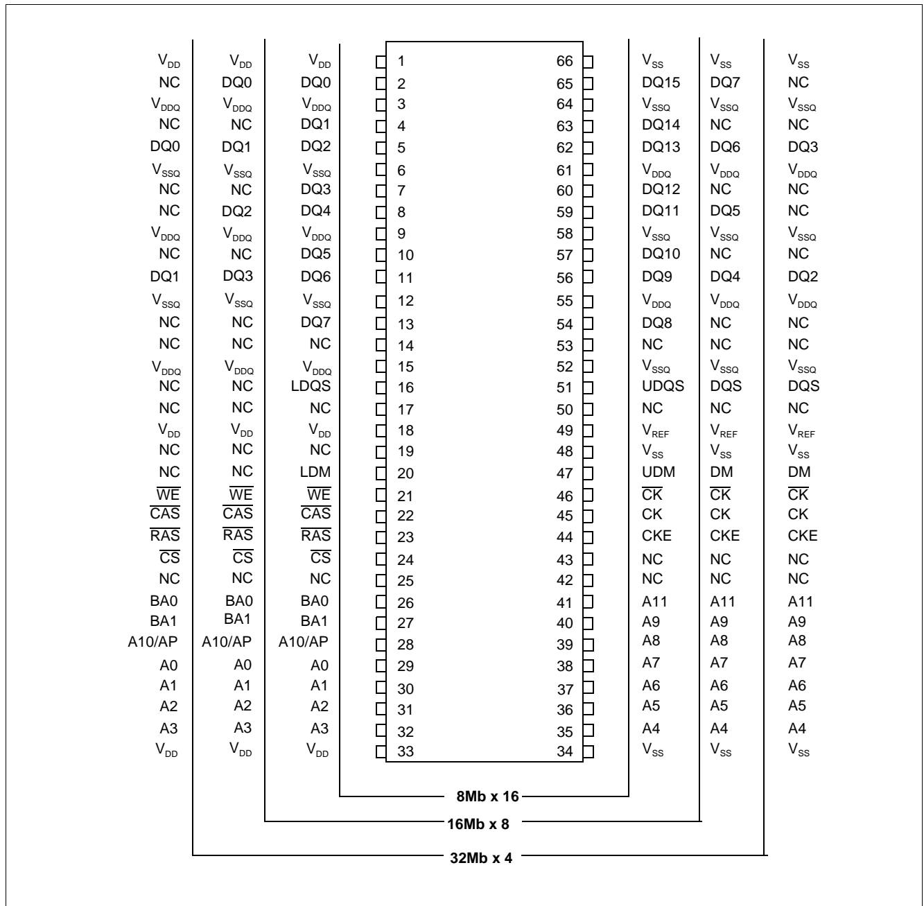
Figure 1 Pin Configuration
