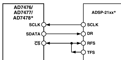
Figure 19. Interfacing to the ADSP-21xx
