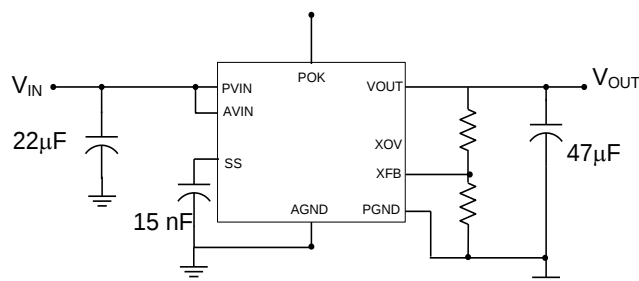
Figure 1. Simple Layout.
