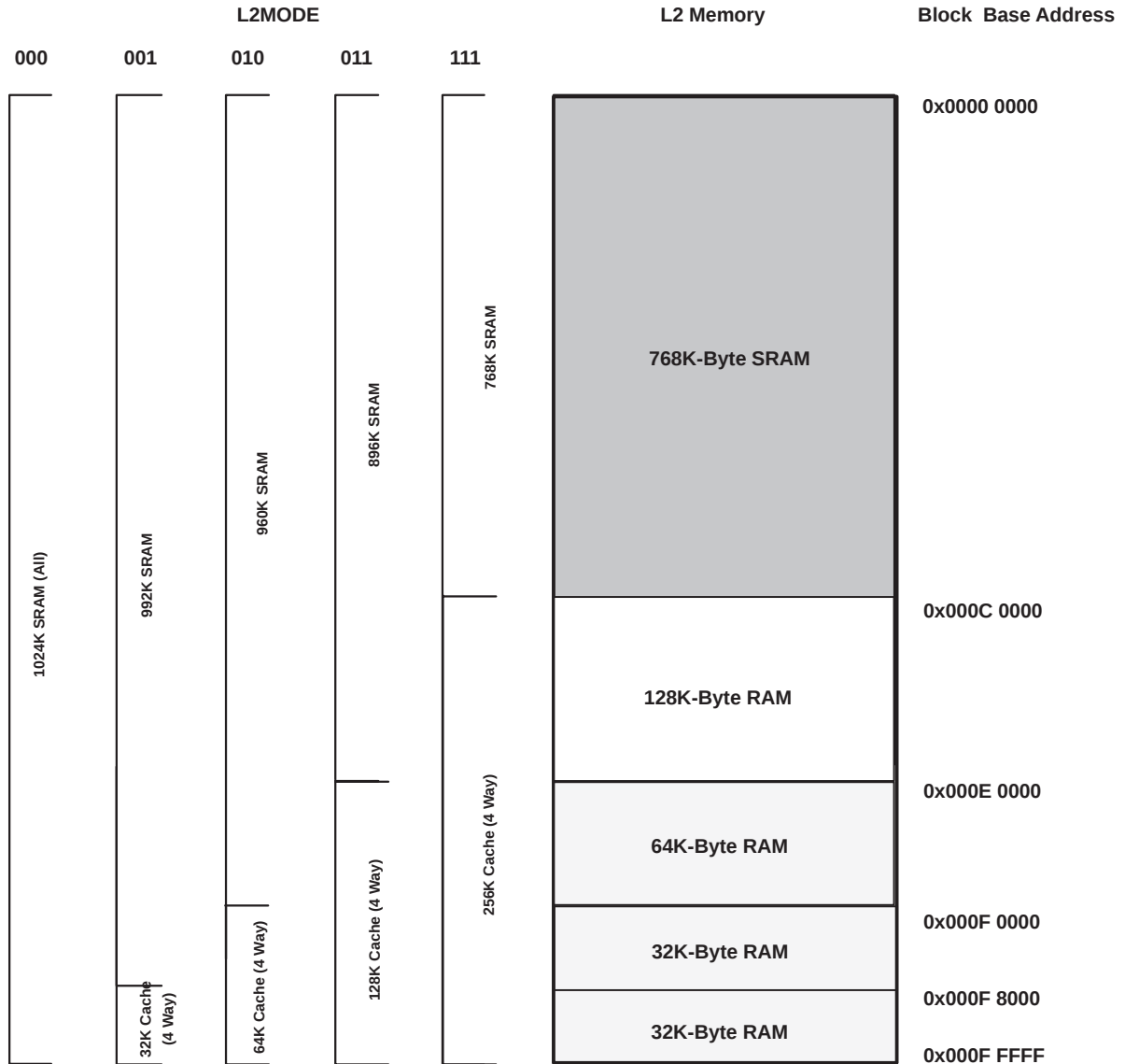
Figure 2. TMS320TCI100 L2 Architecture Memory Configuration
