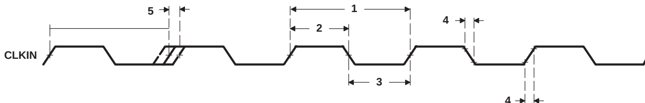
Figure 16. CLKIN Timing
