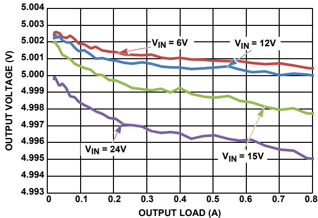
FIGURE 13. V_{OUT} REGULATION vs LOAD, PWM, V_{OUT} = 5V , L_1 = 30\mu H
