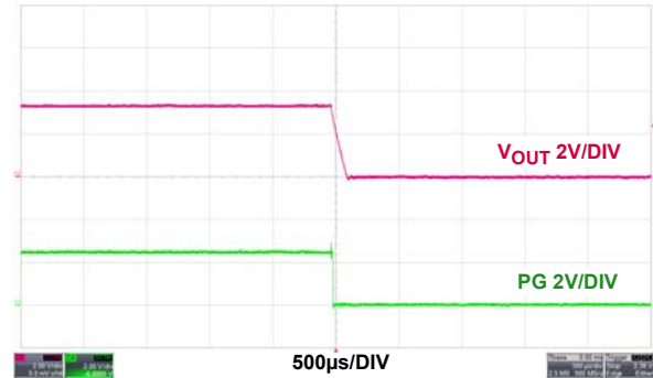
FIGURE 42. OVER-TEMPERATURE PROTECTION, PWM
