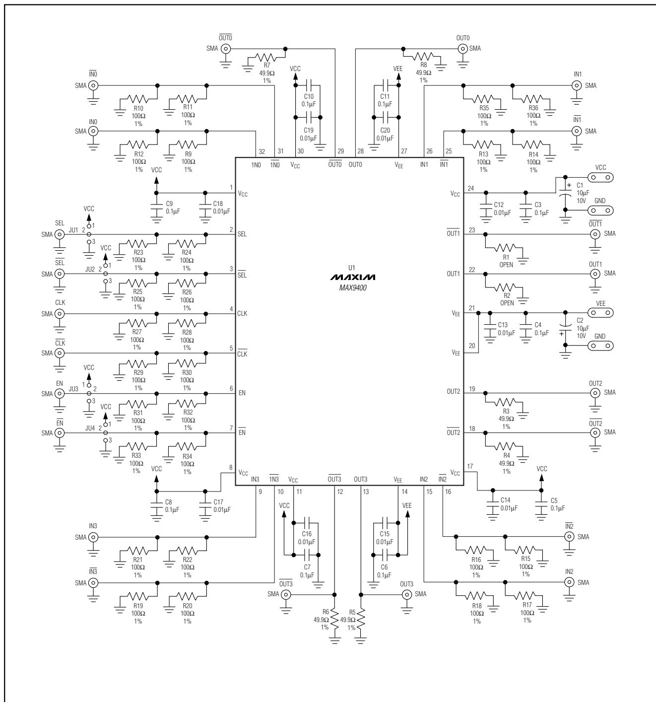
Figure 1. MAX9400 EV Kit Schematic
