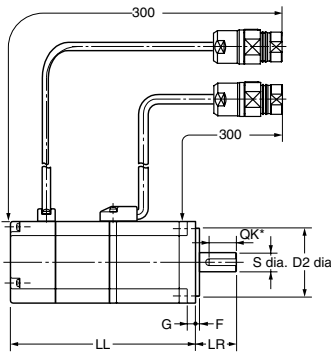
R7M-A□□□30-BS1-D (With brake)
