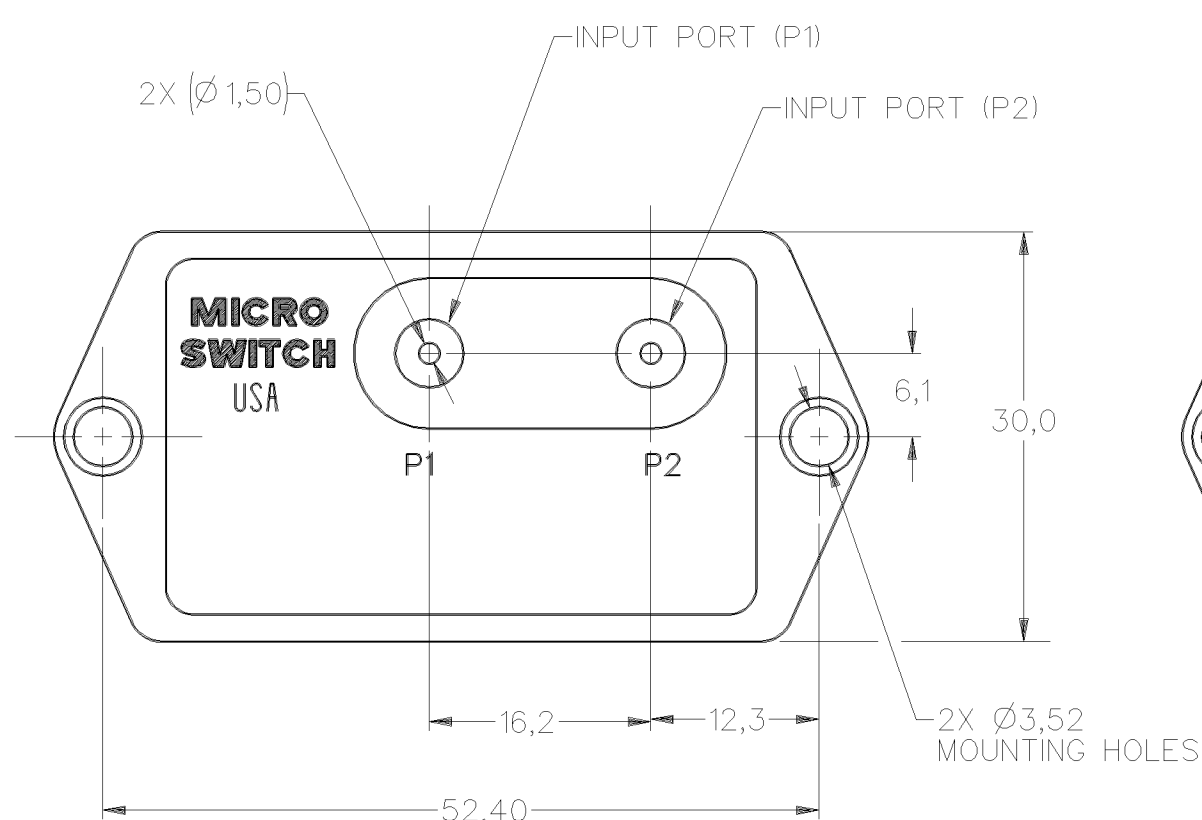
TYPE "D" (DIFFERENTIAL)
