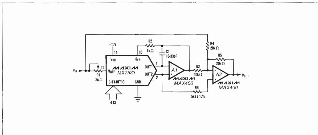
Figure 5. Bipolar Operation (4-Quadrant Multiplication)
