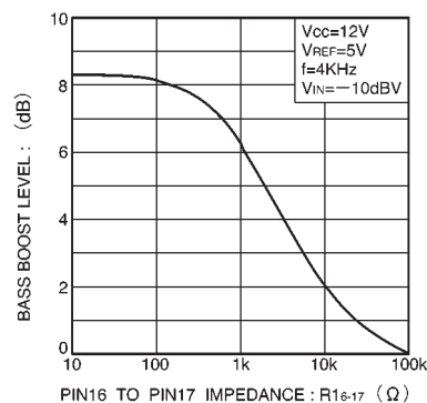
Fig. 5 Bass boost level vs. resistance between pins 16 and 17
