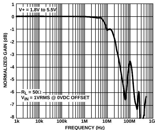
FIGURE 19. FREQUENCY RESPONSE
