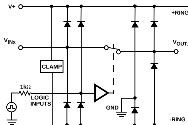
FIGURE 8. OVERVOLTAGE PROTECTION
